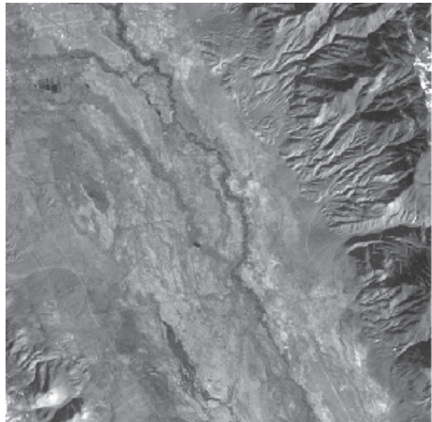
Figure 6-1: Landsat-4 Image
