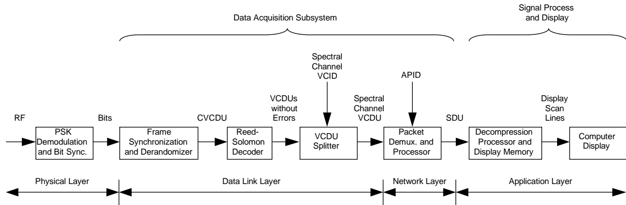
Figure 5-2: Ground Segment
